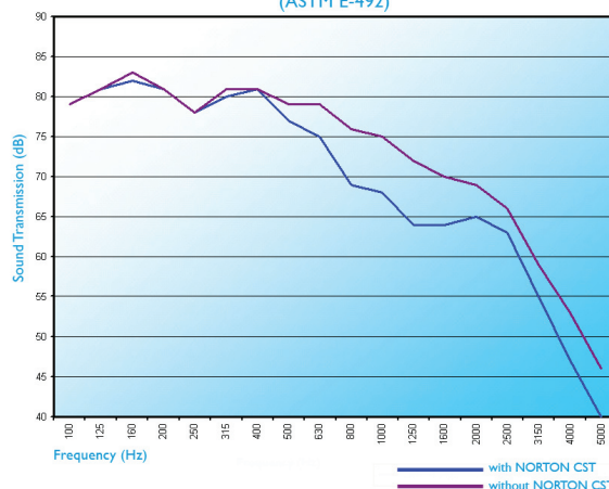
Noise Reduction in a Wood Joist Floor Assembly (ASTM E-492)
